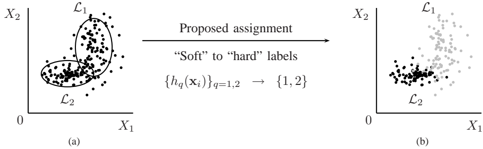
Fig. 3. a) Two Gaussian densities that overlap when the probability for a sample measurement vector \mathbf{x}_i belongs to component q = 1, 2 is h_q(\mathbf{x}_i) ; b) Proposed hard assignment with the help of a random variable, so that clusters \mathcal{L}_1 and \mathcal{L}_2 are the outcome of two Gaussians.
