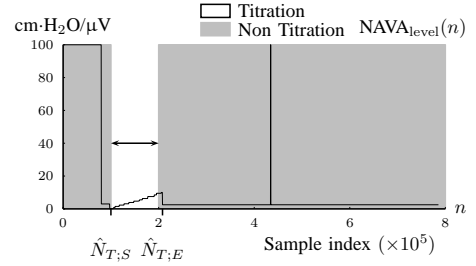
Fig. 6. The result of titration tracking procedure of Figure 5. The lines that belong to \mathcal{G}(\bar{\mu}_1, \Sigma_1) are assigned to the Titration class (Step 1B).
