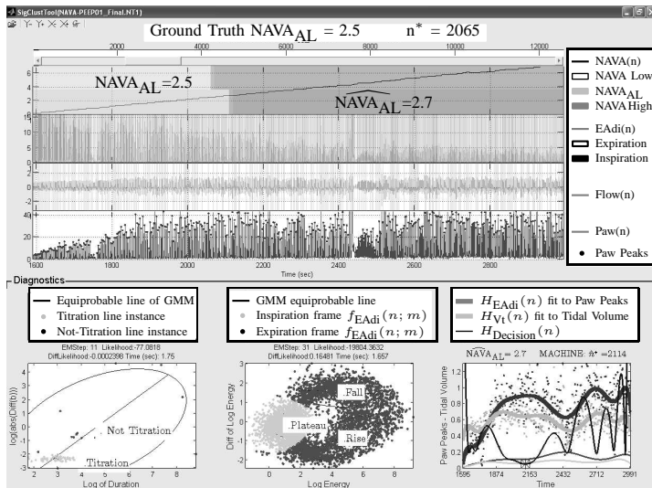
Fig. 13. The graphic interface provides a synopsis of the signal processing steps described in Figures 2, 5, 8, and 11, and allows for real time assessment of how the algorithm identifies NAVA_{AL} . Ground truth NAVA_{AL} denotes the visually estimated adequate NAVA level.
