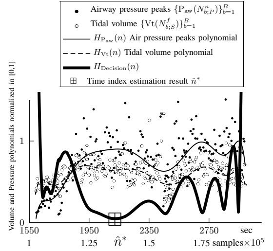
Fig. 11. Time index of plateau, \hat{n}^* , is found when H_{Decision}(n) is minimized, as described in Steps 3 and 4.
