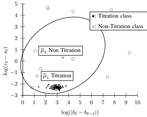
Fig. 5. \text{NAVA}_{\text{level}}(n) titration session tracking by 2 Gaussian components for Figure 4. The component with small dispersion corresponds to Titration class (Step 1B).
