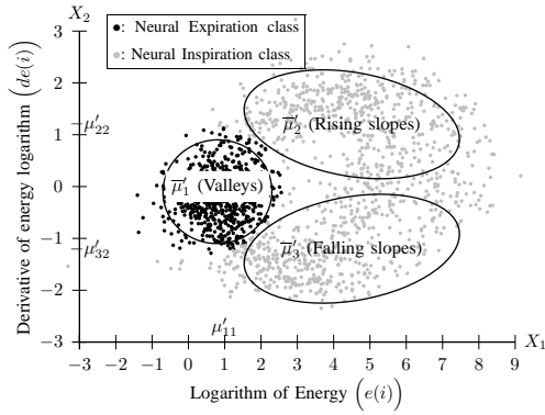
Fig. 8. Clustering of \widehat{\text{EAdi}}(n) frames to Neural Inspiration and Expiration classes (Step 2C).
